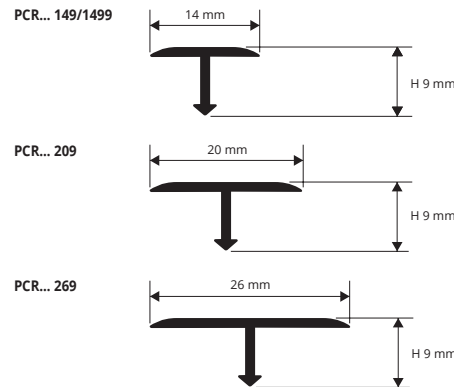
POLISHED BRASS thermo packed - bar length 2,7 lm
