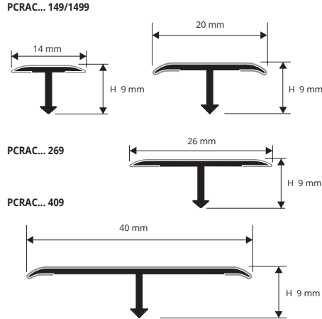
POLISHED STAINLESS ST. AISI 304/1.4301-V2A with protective film - bar length 2,7 lm
