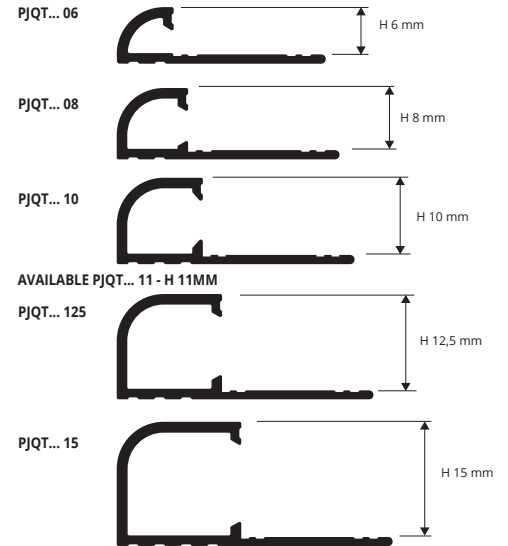
ANODIZED ALUMINIUM (black-grey gun) thermo packed bar length 2,7 lm - pack. 40 Pcs - 108 lm (H 12,5 mm, 15 mm - pack. 20 Pcs)
